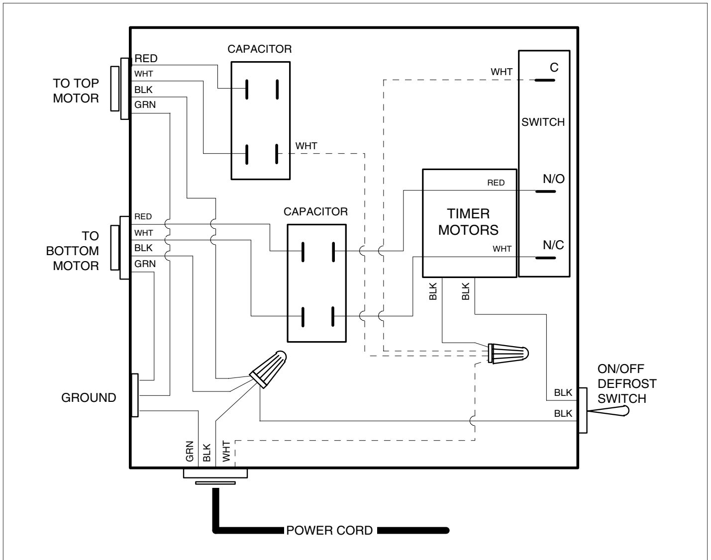
Figure 1 General RA-Series wiring diagram.
